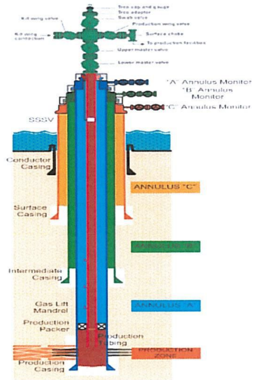
Typical well investigation area
